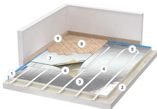
System with floating parquet covering
