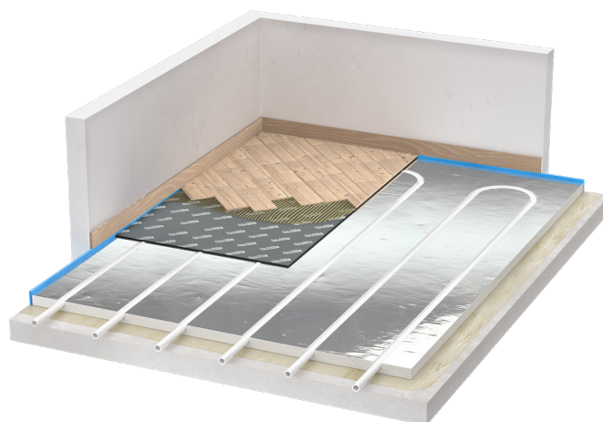
Kilma Futura System with glued parquet covering
