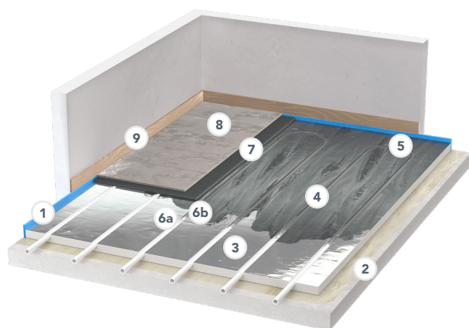
System with glued ceramic covering
