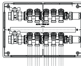
VALVE + 5-WAY + DAMPER
